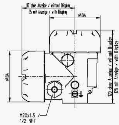
Dual chamber housing, aluminium
