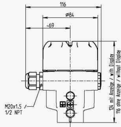
Single chamber housing, aluminium
