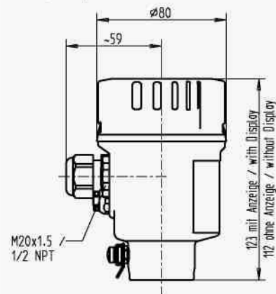
Single chamber housing, stainless steel, deep-drawn
