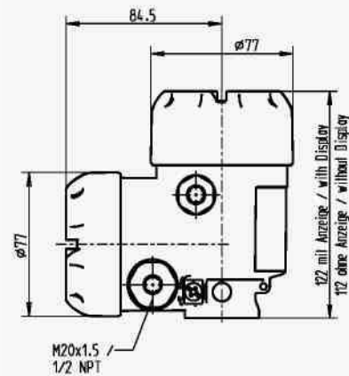
Dual chamber housing, plastic
