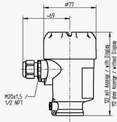
Single chamber housing, plastic
